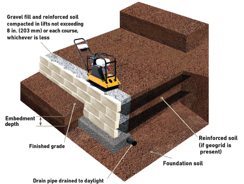
Figure 4: Segmental Wall Construction
