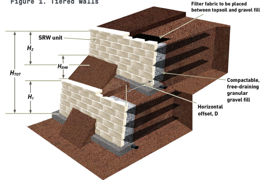
Figure 1. Tiered Walls
