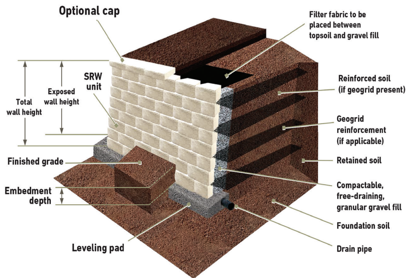
Figure 2: Segmental Wall Components
